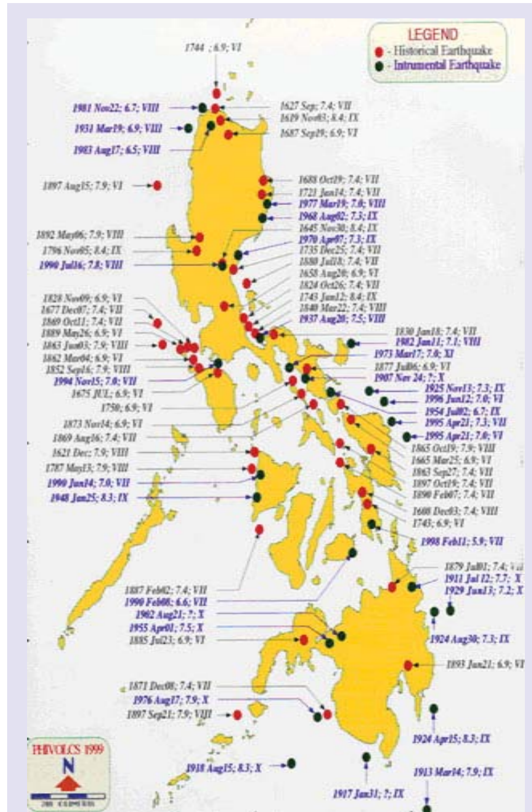
Figure 11: Destructive Earthquakes of the Philippines
