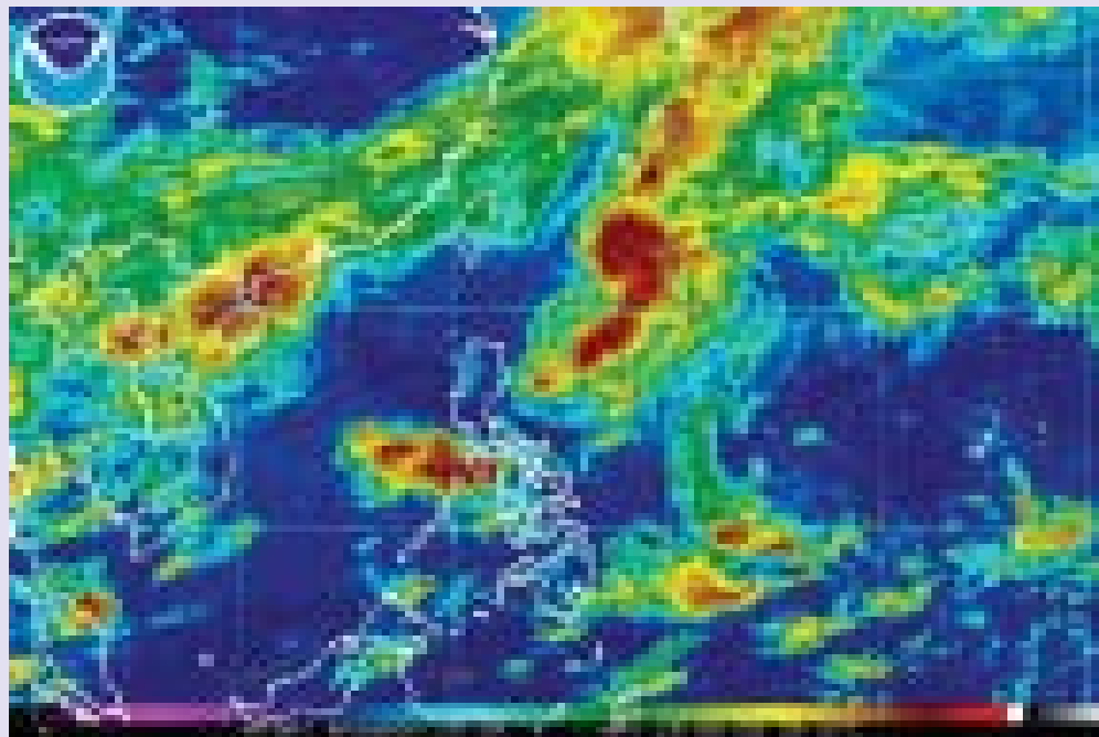
Figure 1: Satellite Map showing typhoons in the area of Philippines
