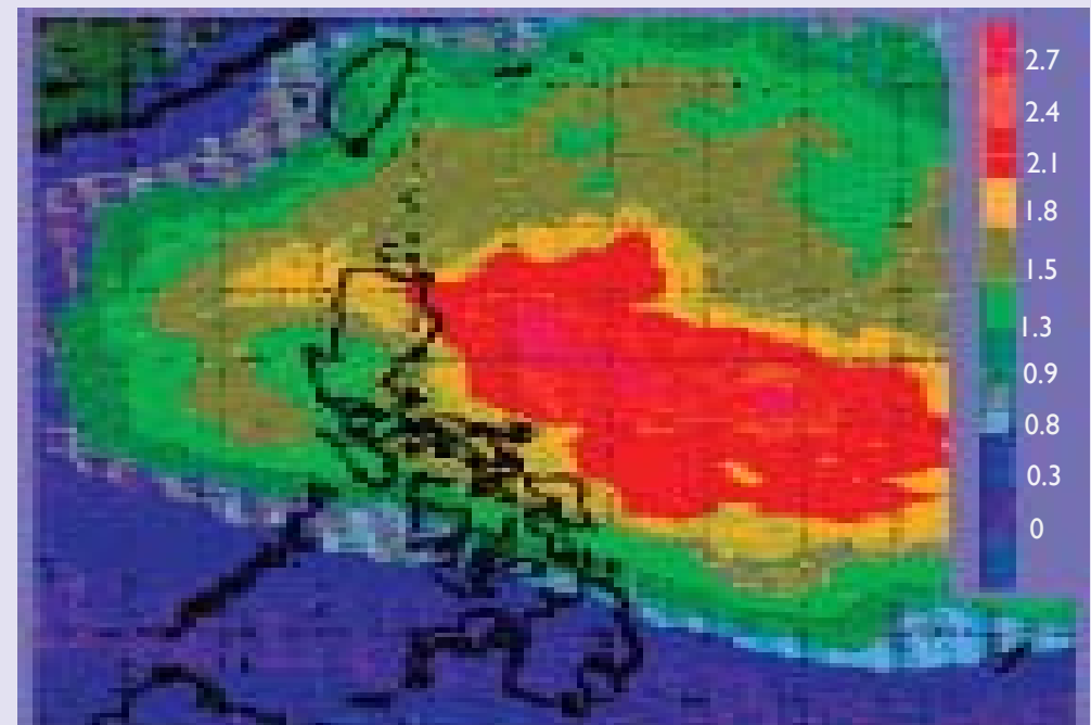
Figure 3: Annual Pattern of Typhoon Incidence from 1950 to 1995. Units indicate typhoon hits. (Source: PAGASA)
